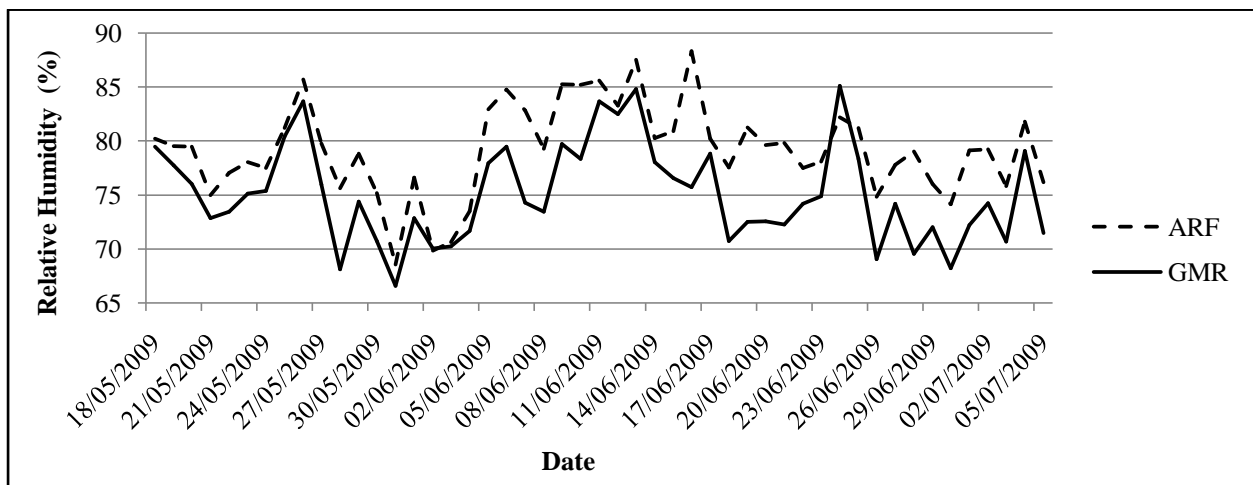
Graphic 2. Relative humidity registered at both environmental stations (EA ARF and EA GMR) used during the night surveys at the Arrecifes sector.
