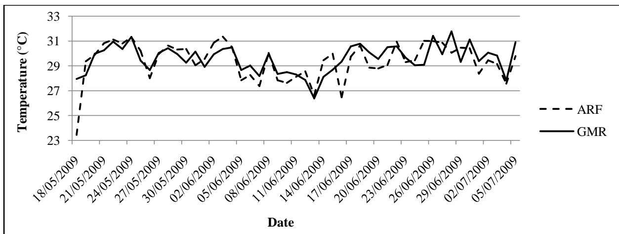
Graphic 1. Temperature registered at both environmental stations (EA ARF and EA GMR) used during the night surveys at the Arrecifes sector.
