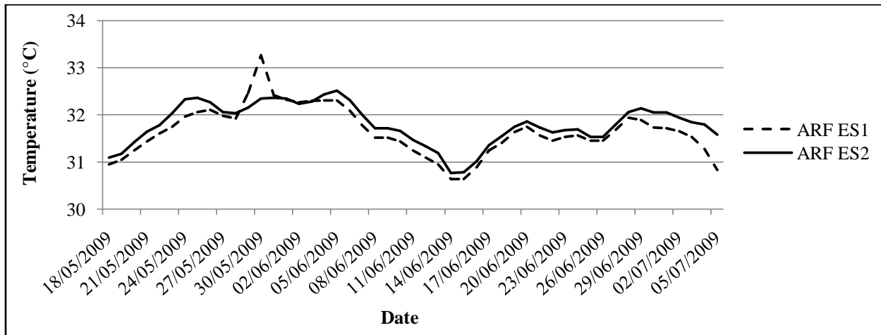
Graphic 3. Average daily temperature registered in the false nest station at Arrecifes beach (ES ARF 1 and 2).
