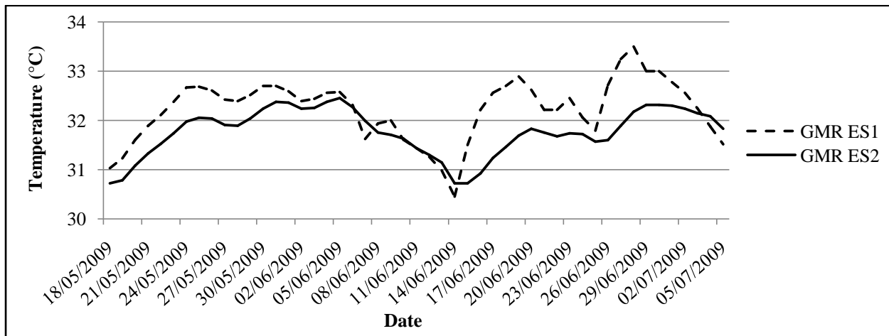
Graphic 5. Average daily temperature registered in the false nest station at La Gumarra beach (ES GMR 1 and 2).
