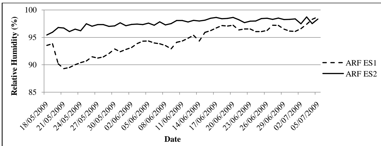
Graphic 4. Average daily relative humidity registered in the false nest station at Arrecifes beach (ES ARF 1 and 2).
